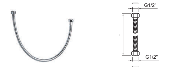
Ref. 97396 L=35cm Ref. 97397 L=60cm
