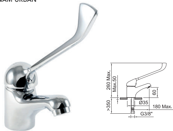
LAVABO CON LEVA GERONTOLOGICA Basin mixer with medical lever
