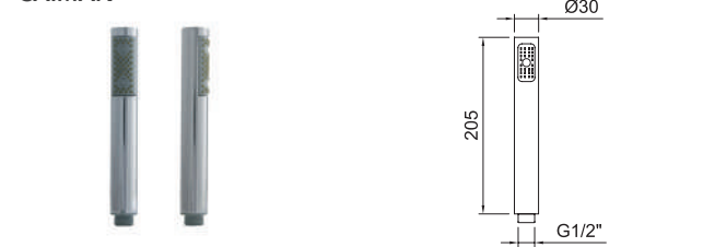
Doccetta Caiman. Caiman shower handset.
