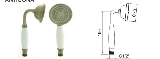
Doccetta Antigona Ø75mm. Antigona shower handset Ø75mm.
