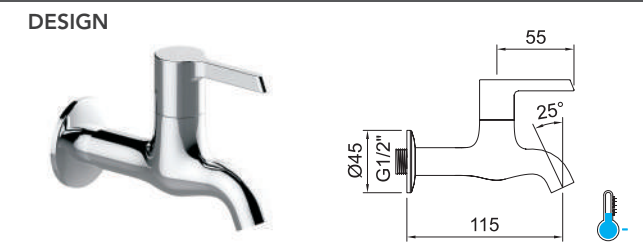
Rubinetto a parete da 1/2". Wall mounted tap 1/2".
