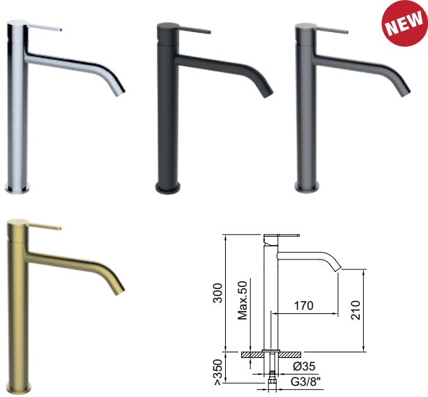
LAVABO 210 Basin mixer 210
