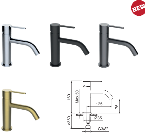
LAVABO 75 Basin mixer 75
