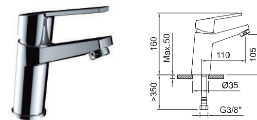
LAVABO 105 Basin mixer 105
