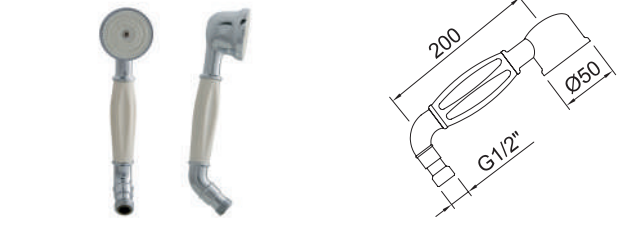
Doccetta Antigona Ø50mm. Antigona shower handset Ø50mm.
