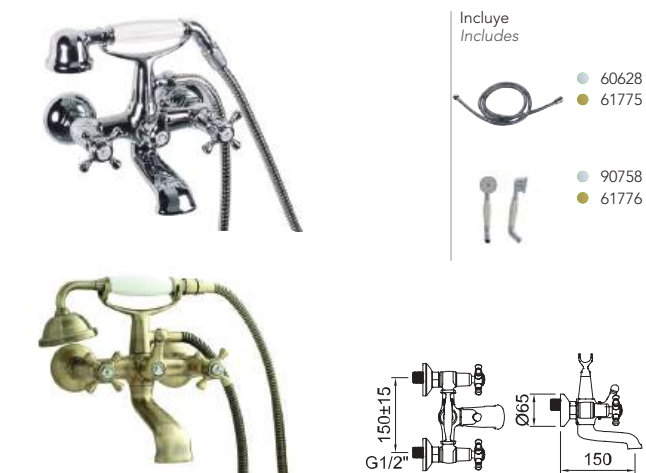
Baño-ducha bimando con inversor manual. Two-handed bath-shower mixer with diverter manual.
