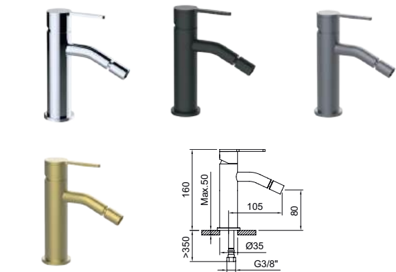
Bidé monomando con aireador a rótula y flexibles 3/8" >350mm. Single-lever bidet mixer with swivel aerator and flexible hoses 3/8" >350mm.
