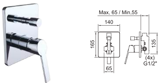
Ducha monomando empotrar 1/2". Concealed single-lever shower mixer 1/2".
