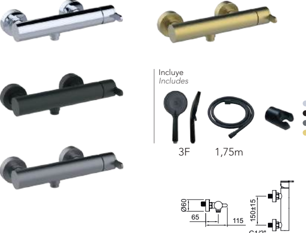
Ducha monomando. Single-lever shower mixer.
