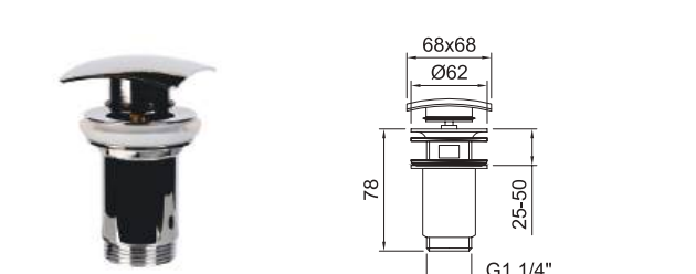
Válvula descarga sistema click-clack universal 1 1/4". Pop-up quick-clac universal 1 1/4".
