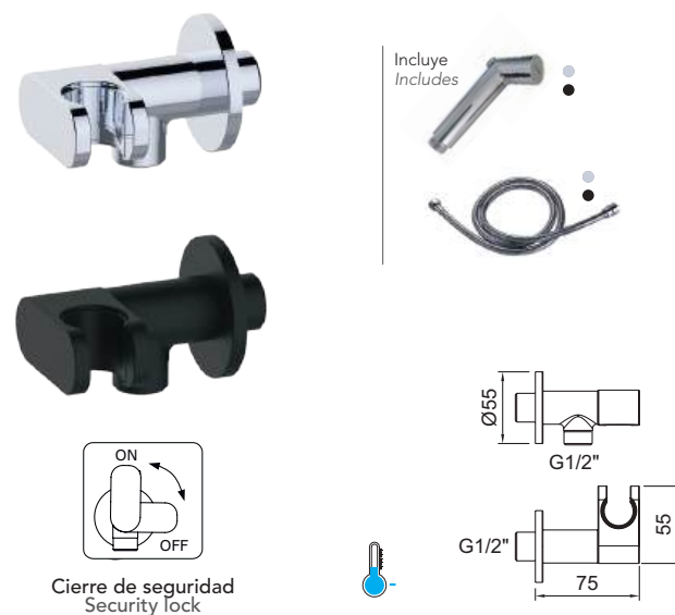
Ducha higiénica mural con soporte integrado. Wall mounted shattaf with support included.
