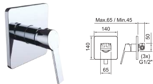
Ducha monomando empotrar 1/2". Concealed single-lever shower mixer 1/2".
