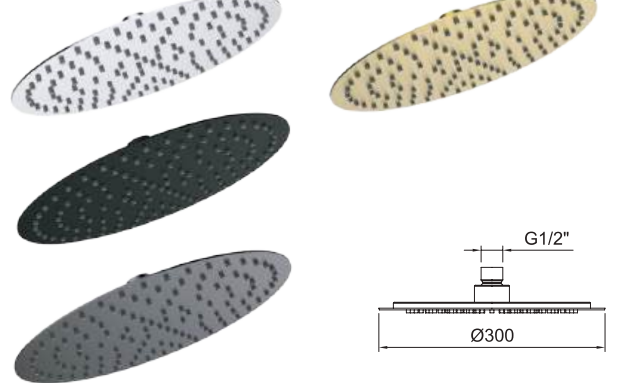
Rociador ducha Slim Inox Air Ø300mm. Slim Inox Air head shower Ø300mm.
