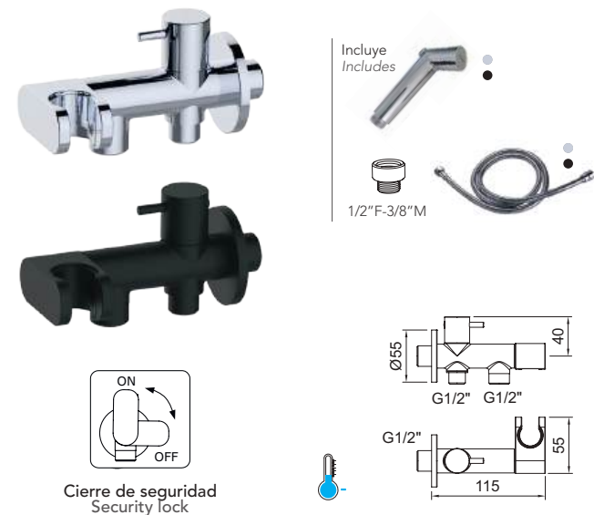
Ducha higiénica mural con salida cisterna. Wall mounted shattaf with water tank outlet.
