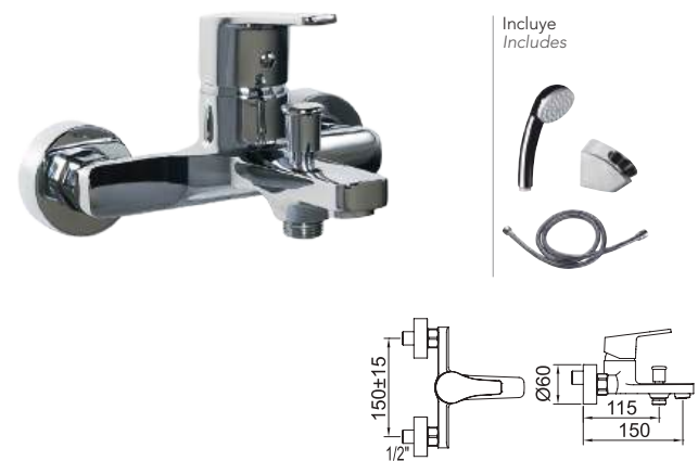
Baño-ducha monomando con aireador e inversor. Single-lever bath-shower mixer with aerator and diverter.
