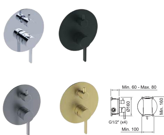
Ducha monomando empotrar 1/2". Concealed single-lever shower mixer 1/2".
