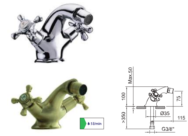
Bidé bimando con aireador a rótula y flexibles 3/8" >350mm. Two-handed bidet mixer with swivel aerator and flexible hoses 3/8" >350mm.
