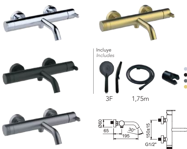
Baño- ducha monomando con aireador e inversor cerámico. Bath-shower mixer single-lever with aerator and ceramic diverter.
