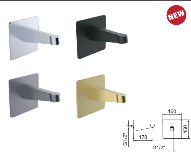
Brazo de rociador mural. Wall-mounted arm shower.
