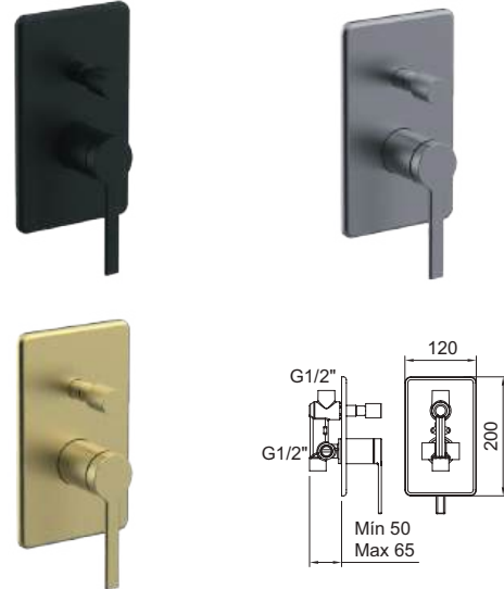
Ducha monomando empotrar 1/2". Concealed single-lever shower mixer 1/2".
