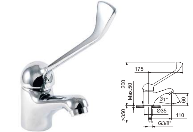
LAVABO CON LEVA CLINICA Basin mixer with medical lever PANAM URBAN
