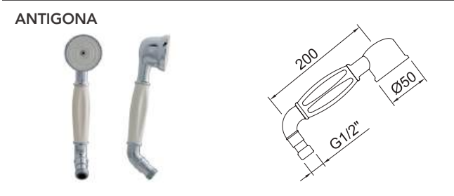
Doccetta Antigona Ø50mm. Antigona shower handset Ø50mm.
