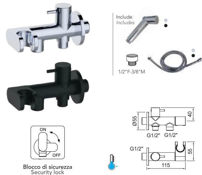
Doccia igienica a parete con scarico WC. Wall mounted shattaf with water tank outlet.
