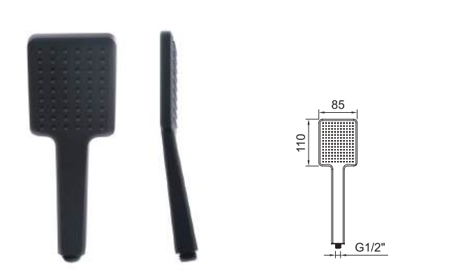
Doccetta Nine Xtreme 85x110mm. Nine Xtreme shower handset 85x110mm.
