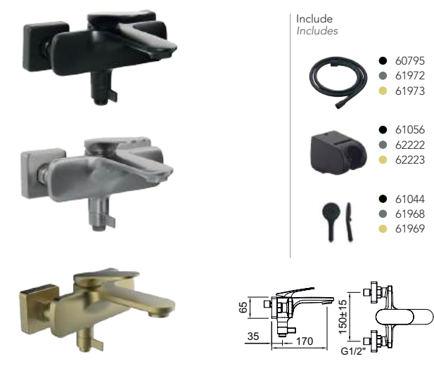
Vasca con doccia monocomando. Single-lever bath-shower mixer with aerator and ceramic diverter.
