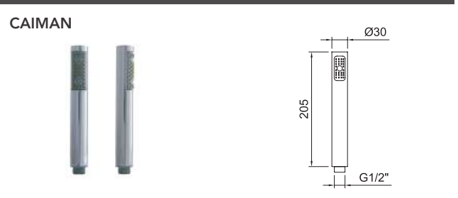
Doccetta Caiman. Caiman shower handset.
