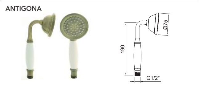
Doccetta Antigona Ø75mm. Antigona shower handset Ø75mm.
