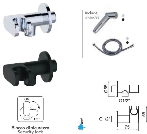
Doccia igienica a parete con supporto integrato. Wall mounted shattaf with support included.
