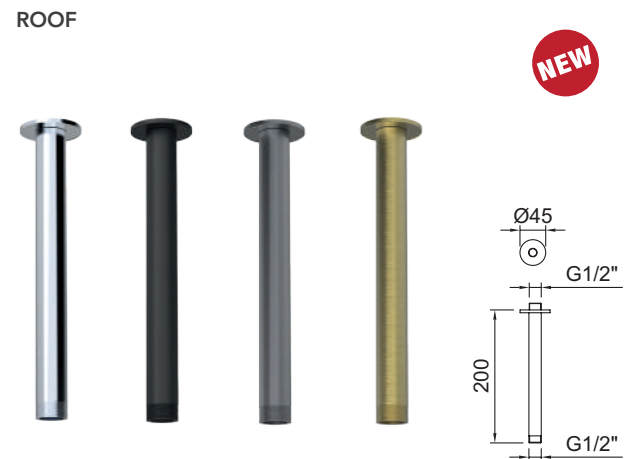
Braço de chuveiro tecto Roof 200mm. Roof ceiling arm shower 200mm.
