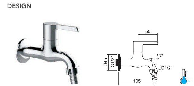
Torneira mural 1/2" com acessório mangueira. Wall mounted tap 1/2" with hose fitting.
