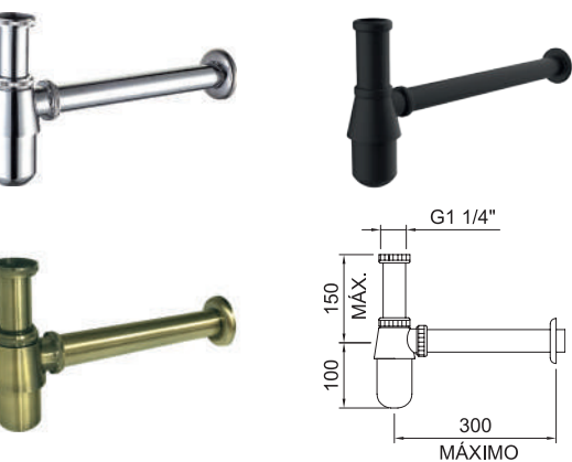
Sifão garrafa 1 1/4" com tubo de Ø32mm. Bottle trap 1 1/4" with tube Ø32mm.
