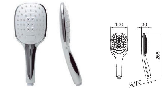
Chuveiro de mão Style 100x120mm. Style shower handset 100x120mm.
