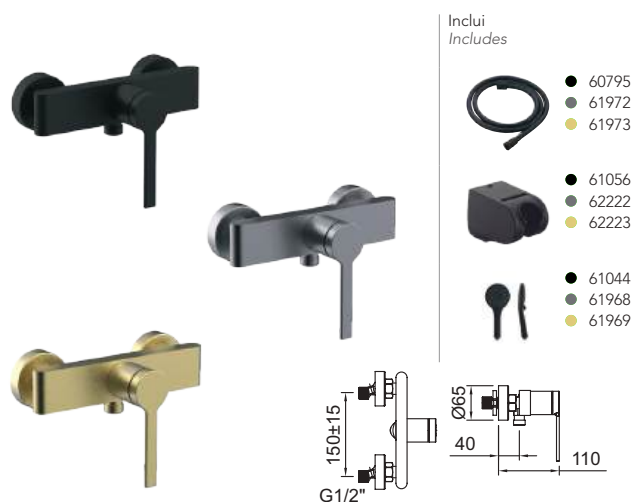
Duche monocomando. Single-lever shower mixer.
