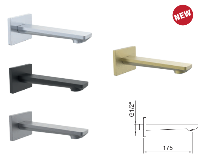
Cano banheira mural. Bath spout.
