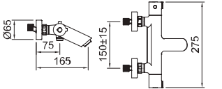
Banheira-duche termostática com areador e inversor incorporado no manípulo de caudal. Thermostatic bath-shower mixer with aerator and integrated shower diverter.
