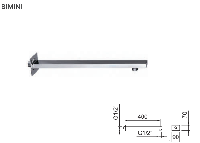
Braço de chuveiro mural Bimini 400mm. Bimini wall-mounted arm shower 400mm.
