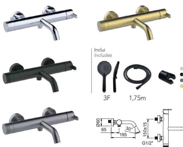
Banheira-duche monocomando com areador e inversor cerâmica. Bath-shower mixer single-lever with aerator and ceramic diverter.
