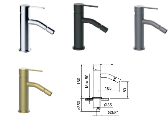
Bidé monocomando com areador orientável e flexíveis 3/8" >350mm. Single-lever bidet mixer with swivel aerator and flexible hoses 3/8" >350mm.
