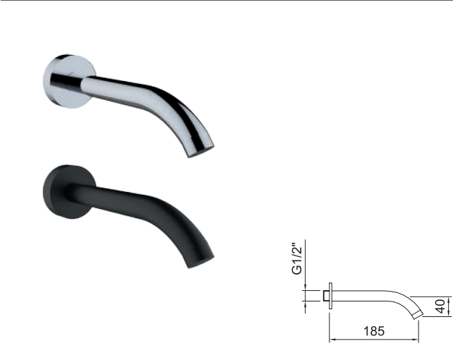
Cano mural Caiman. 185mm Bath spout Caiman. 185mm
