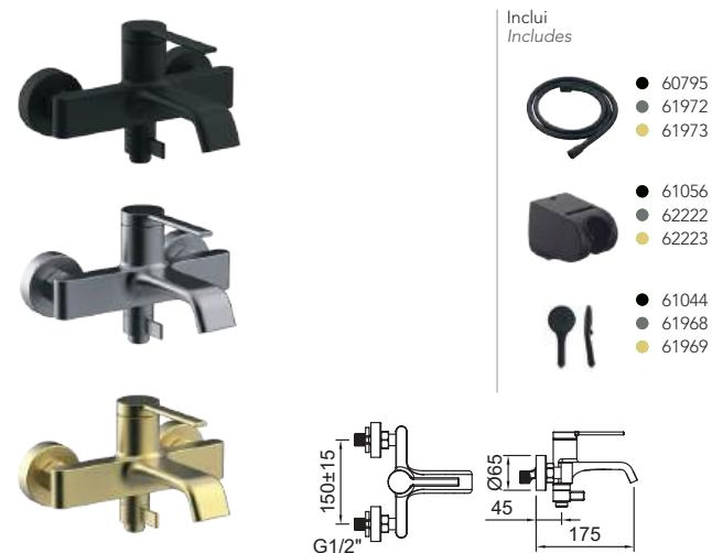
Banheira-duche monocomando com areador e inversor cerâmica. Single-lever bath-shower mixer with aerator and ceramic diverter.
