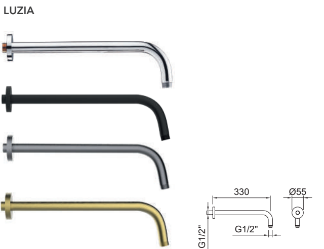
Braço de chuveiro mural Luzia 330mm. Luzia wall-mounted arm shower 330mm.
