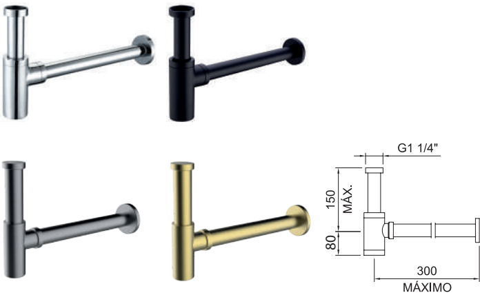
Sifão garrafa 1 1/4" com tubo de Ø32mm. Bottle trap 1 1/4" with tube Ø32mm.
