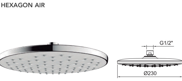
Chuveiro Hexagon Air Ø230mm. Hexagon Air head shower Ø230mm.
