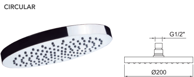
Chuveiro Circular Ø200mm. Circular head shower Ø200mm.
