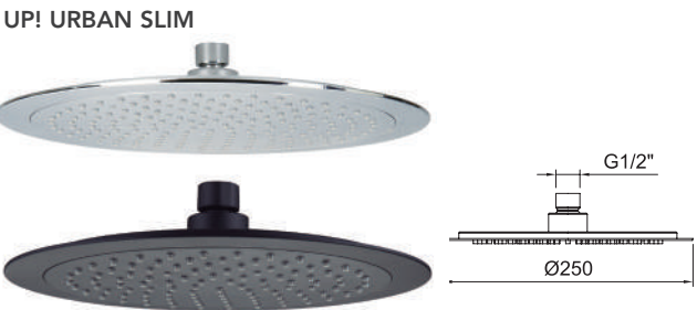
Chuveiro Up! Urban Slim Ø250mm. Up! Urban Slim head shower Ø250mm.
