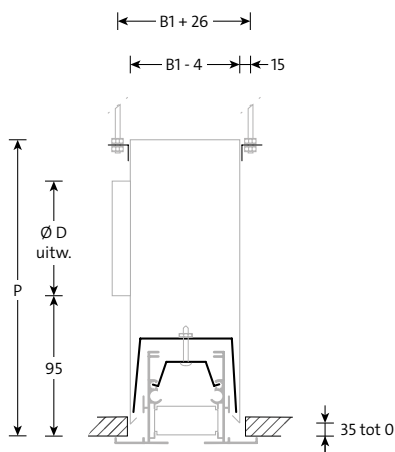
click-in plenumbox sparingmaat = B1
