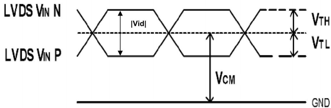
Fig 4.1 LVDS characteristics
