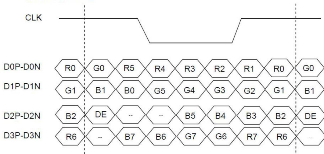
Figure 5.3 LVDS data input format (VESA standard)
