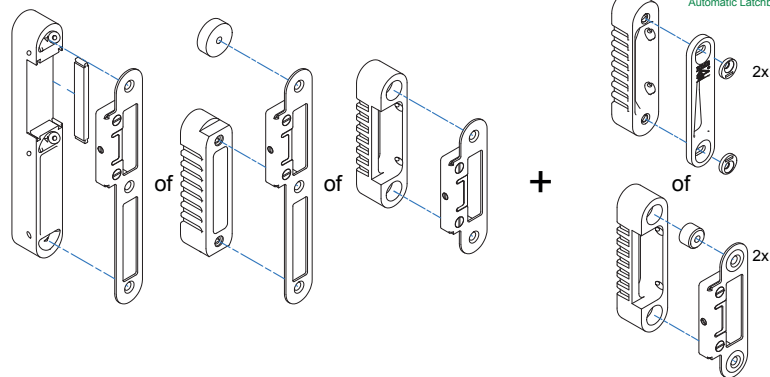
Sluitkom Dagschoot Art. nr. 707021 Casing for Adjustable Strike Latchbolt Magneet t.b.v. Automatic Dagschoot Art. 200089 (8 mm) Art. 200179 (10 mm) Magnet for Adjustable Strike Automatic Latchbolt
