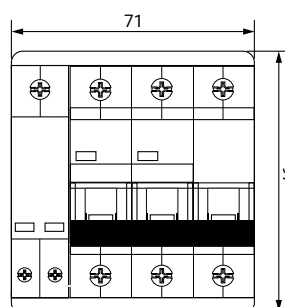
COMBI-2PT
