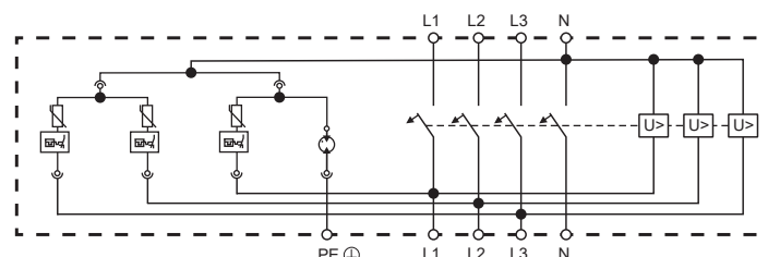
COMBI-4PT
