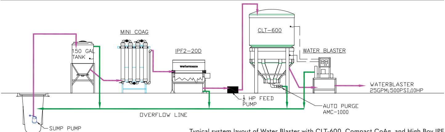
Typical system layout of Water Blaster with CLT-600, Compact CoAg, and High Boy IPF
