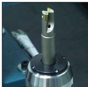
Coolant-thru tool installed
