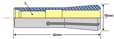
SlimFIT Collet Style
